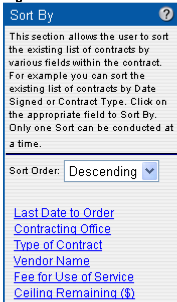
Figure 100. Sort Selections
